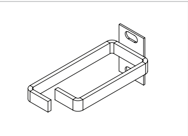
Metal Cable Management Rings ICCMSCMPR1 1.70" Single, Vertical ICCMSCMPR2 3" Single, Vertical
